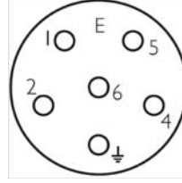
Mating Connector: LPA06BFRDN170 PIN Arrangement
